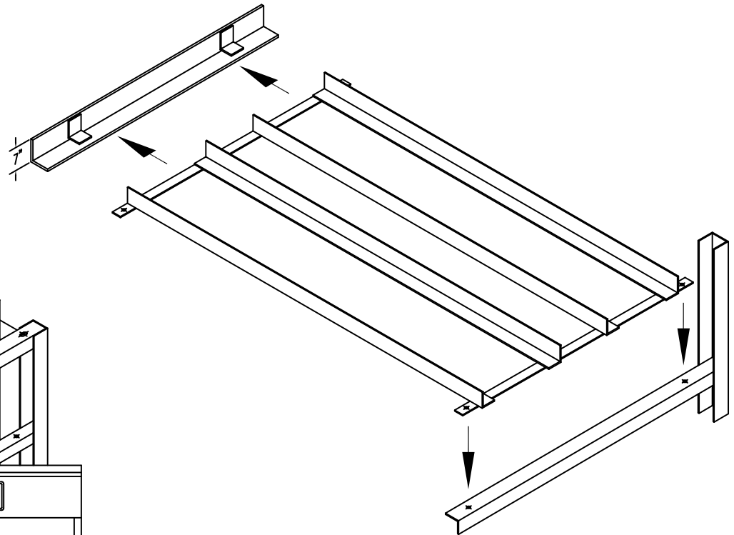
TANK TRAY DETAIL NOT REQUIRED ON VERTICAL CYLINDER CAGE
