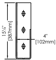
LIFTOUT RAIL BRACKET-RH (131076)
