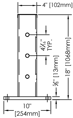
SINGLE RAIL POST (131103)
