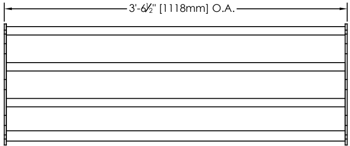
4' RAIL (131046)
