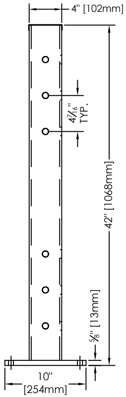
DOUBLE RAIL POST (131123)
