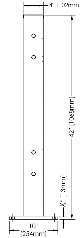
DOUBLE RAIL POST (133123)
