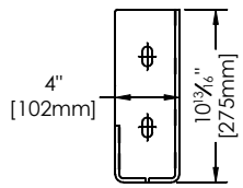
LIFTOUT RAIL BRACKET-LH (133075)
