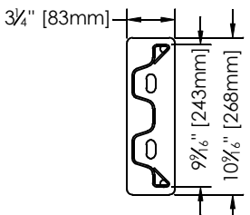
11 GA. MATERIAL - RAIL 1/4" MATERIAL - ENDS
