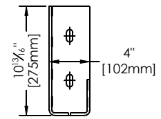
LIFTOUT RAIL BRACKET-RH (133076)
