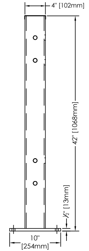
DOUBLE RAIL POST (133123)
