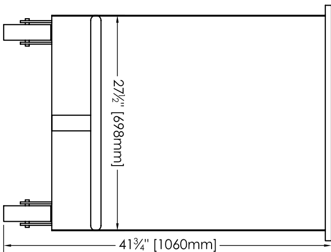
BACK ELEVATION
