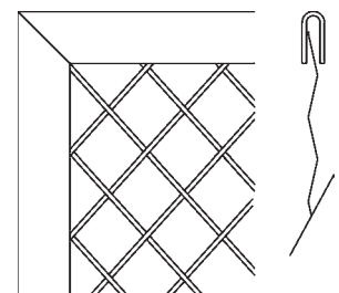
1 1/2" x 16 gauge U-edging with 2" reveal.
